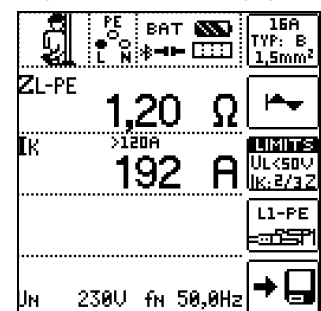
Loop Resistance Meas. Display
